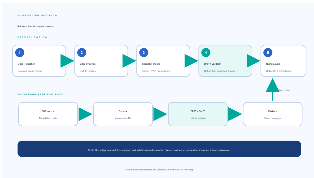
Figure — Data-flow diagram: selected case evidence and retrieved knowledge converge in a validated advisory report before a named human records the next step.
